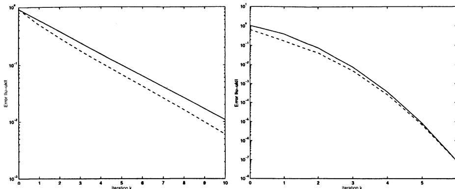
FIGURE 2. Linear convergence on long time intervals on the left and superlinear convergence on short time intervals on the right. Dashed the numerical results and solid the derived upper bounds for the convergence rate
