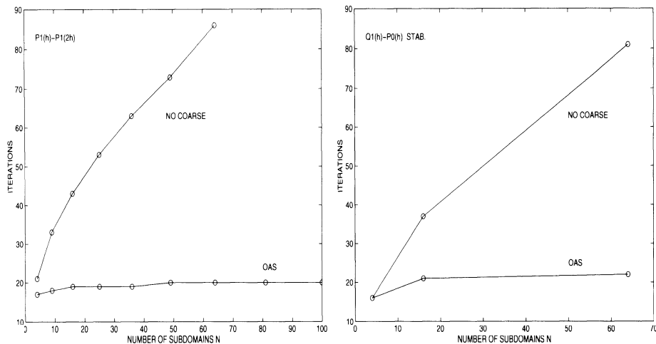
FIGURE 2. Iteration counts for GMRES with overlapping additive Schwarz preconditioner \widehat{K}_{OAS}^{-1} (with and without coarse problem): subdomain size H/h = 8 , overlap \delta = 2h , Stokes problem with P_1(h) - P_1(2h) finite elements (left), lid-driven cavity Stokes flow with Q_1(h) - P_0(h) stab. elements (right).
