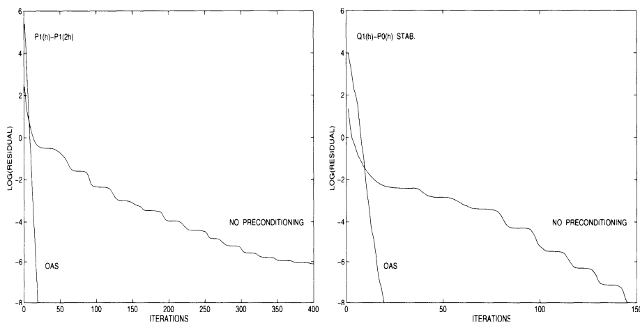
FIGURE 3. Convergence history for GMRES with and without overlapping additive Schwarz preconditioner \widehat{K}_{OAS}^{-1} : N = 16 , subdomain size H/h = 8 , overlap \delta = 2h , Stokes problem with P_1(h) - P_1(2h) finite elements (left), lid-driven cavity Stokes flow with Q_1(h) - P_0(h) stab. elements (right).
