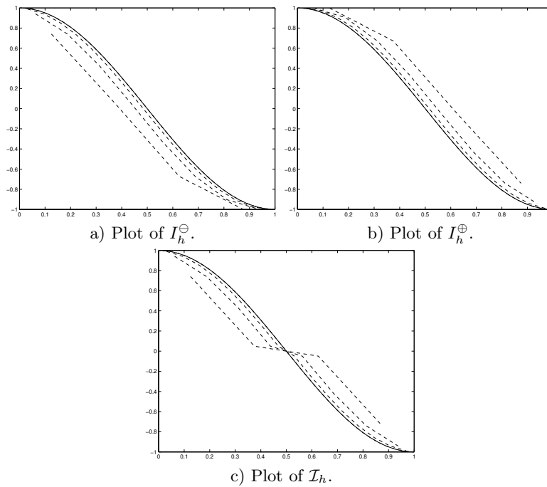
Fig. 1. Plots of the interpolation operators over a sequence of refined meshes. If the mesh is refined, the interpolation I_H^{\ominus} v increases, while I_H^{\oplus} v decreases. The interpolation \mathcal{I}_H v increases in \Omega^+ and decreases in \Omega^- . I_H^{\ominus} v is always below v , while I_H^{\oplus} v is always above v . \mathcal{I}_H v is below v in \Omega^+ and above v in \Omega^- .
