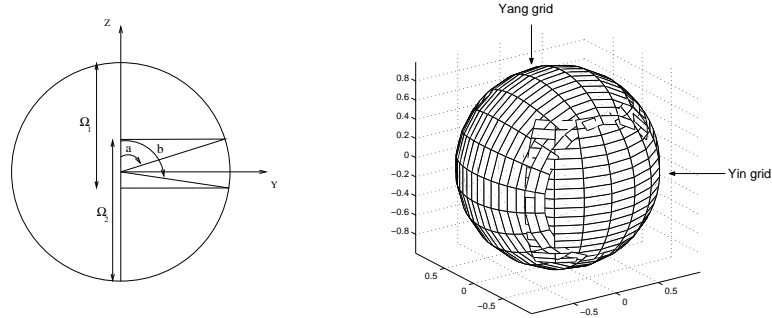
Fig. 1. Left: Two overlapping subdomains. Right: The Yin-Yang grid system.
