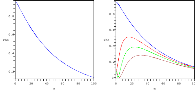
Fig. 2. Left: Behavior of the convergence factor \rho_{cla} . Right: Comparison between \rho_{cla} (top curve), \rho_{T0} ( 2^{nd} curve), \rho_{T2} ( 3^{th} curve) and \rho_{O0} (bottom curve). In both plots a = \pi - L/2 and the overlap is L = b - a = \frac{1}{100} and \eta = 2 .
