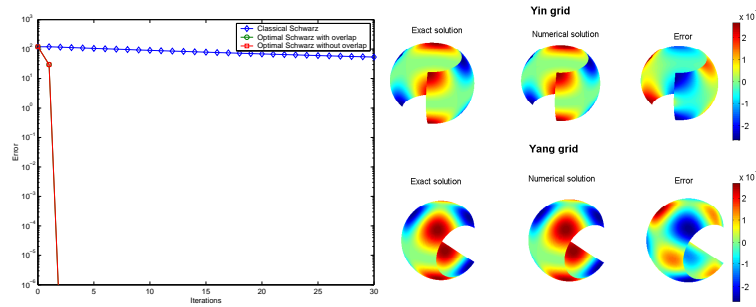
Fig. 3. Left: Convergence behavior for the methods analyzed for the two subdomain case. Right: Screenshots of solutions and the error in the Yin-Yang grid system.
