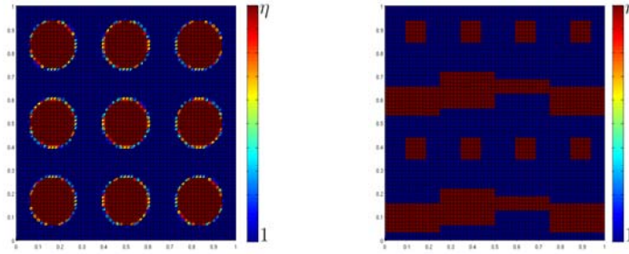
Fig. 2. Left: Coefficient corresponding to nine high-contrast inclusions. Light grey indicates the high-contrast part, \kappa(x) = \eta . Dark grey indicates value \kappa(x) = 1 . The results are displayed in Table 2 and the degrees of freedom information in Table 1. Right: Coefficient with inclusions and long channels. See Tables 1 and 3.
