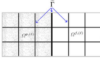
Fig. 1. Global interface \tilde{\Gamma} that includes all local interfaces and the Stokes/Darcy interface \Gamma .
