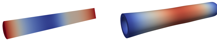
Fig. 7 Pressure and deformation at time t = 0.007 s. The deformation is magnified by a factor of 10.
