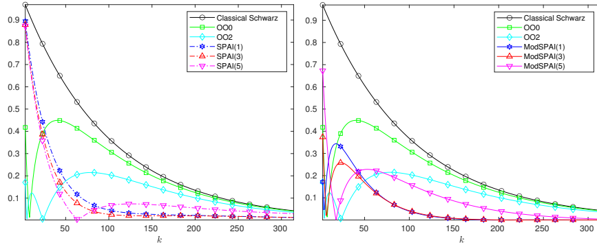
Fig. 1: Comparison of the convergence factors as function of the Fourier frequency k for the classical Schwarz method, algebraic SPAI transmission conditions (left) and the modified SPAI transmission conditions (right).
