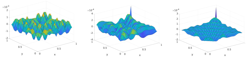
Fig. 1 Greens function for 3 Helmholtz problems. Left: closed cavity; middle: wave guide; right: free space, where optimized Schwarz solvers are as effective as for Laplace problems [6].
