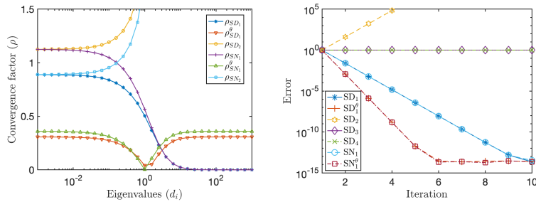
Fig. 2 Convergence factor as a function of eigenvalues (left) and error decay as a function of the number of iterations (right).
