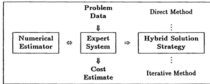
Fig. 1 Adaptive iterative solver. Reproduced from [38] with permission.
